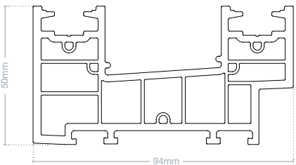
Outer frame EWS 7050
