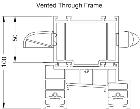
Vented Through Frame
